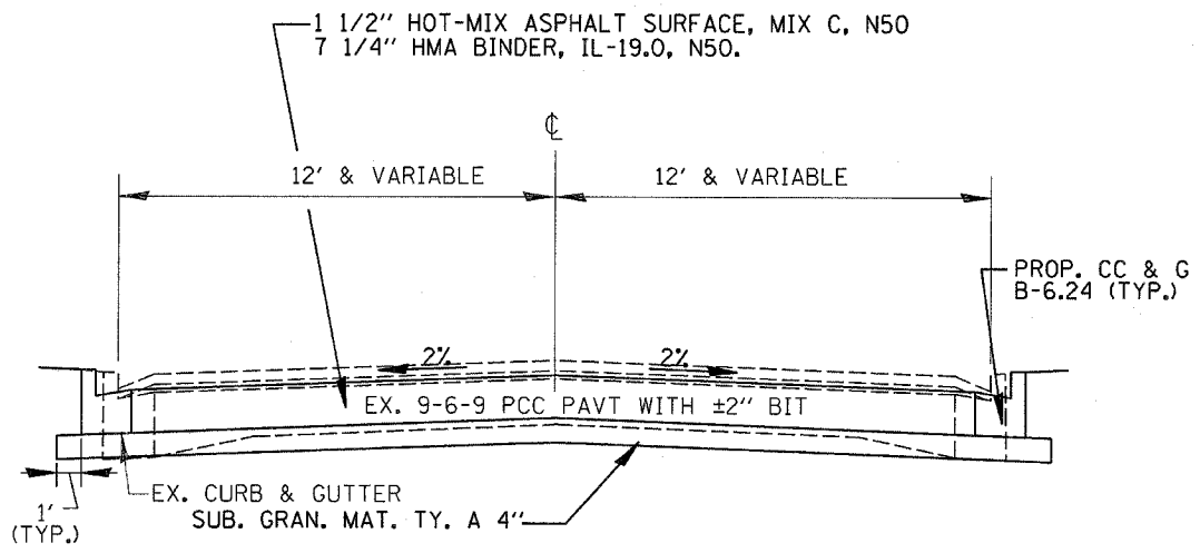
TYPICAL SECTION TODD STREET STA. 223+90 TO STA. 225+87
