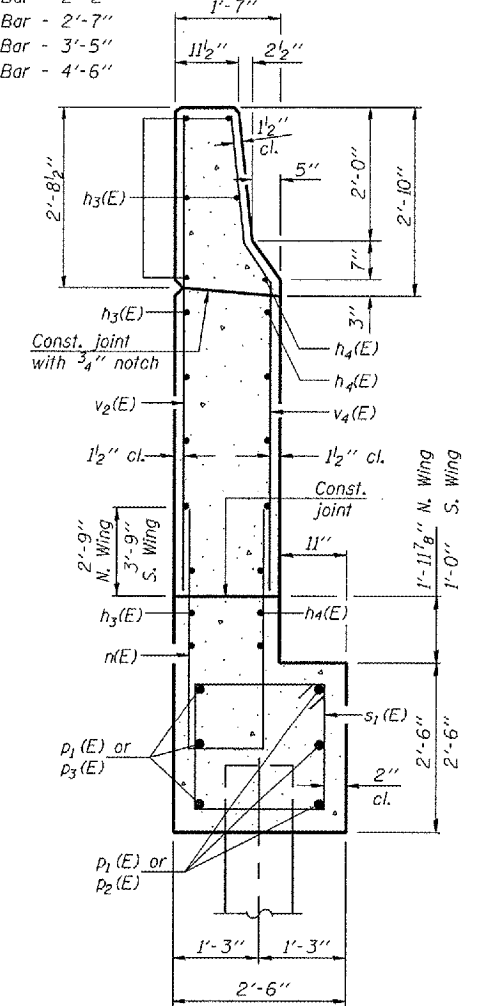
SECTION C-C
