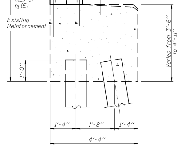
SEC. THRU EXISTING ABUT.
