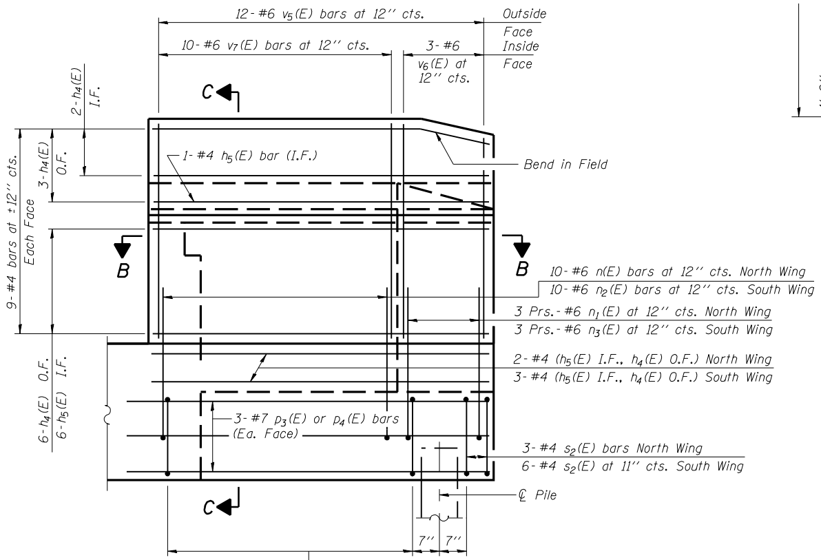
WING WALL ELEVATION Showing Reinforcement
