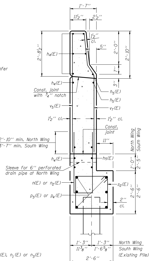
SECTION C-C
