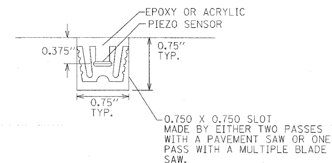
PIEZO SENSOR INSTALLATION DETAIL
