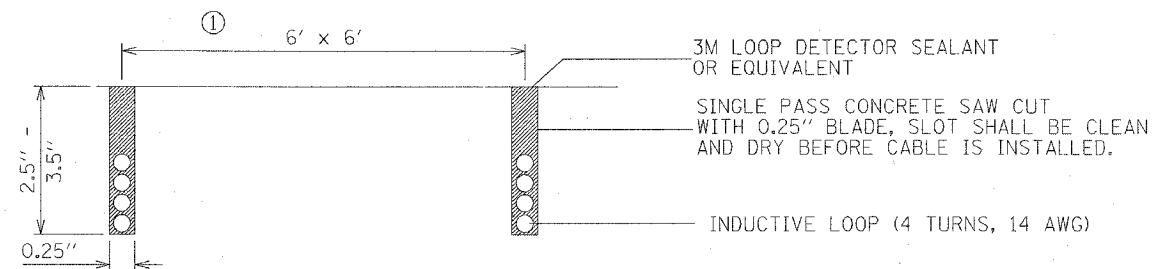
SECTION A - A - LOOP DETAIL
