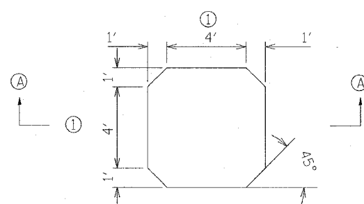
LOOP DIMENSION DETAIL
