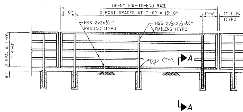
TYPICAL ELEVATION
