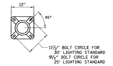
ANCHOR BASE DETAIL
