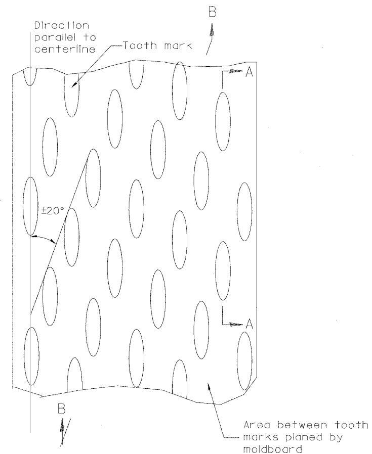
PLAN
