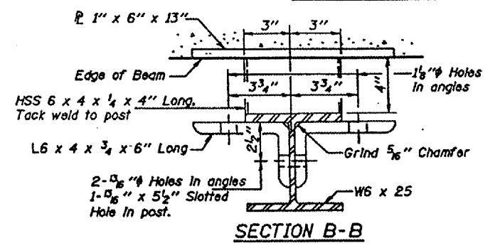
SECTION AT RAIL POST
