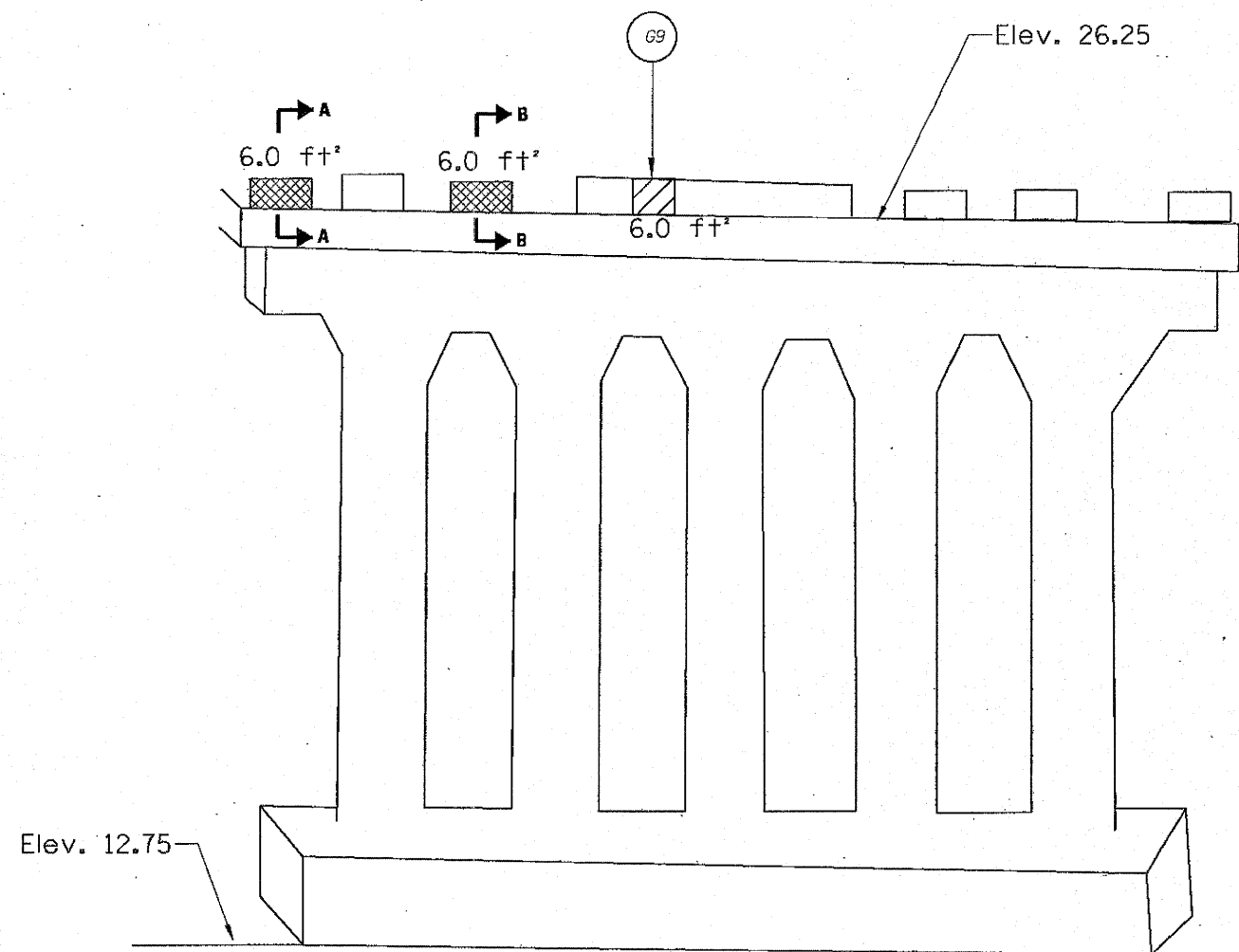
PIER NO. 9- ELEVATION VIEW LOOKING WEST
