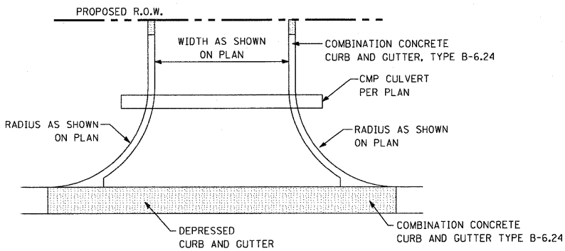
CURB AND GUTTER SECTION
