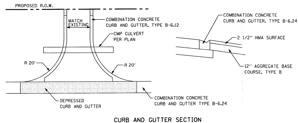
CURB AND GUTTER SECTION
