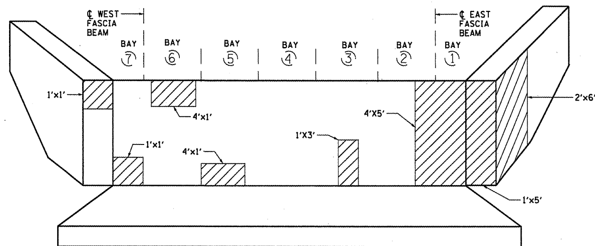
NORTH ABUTMENT
