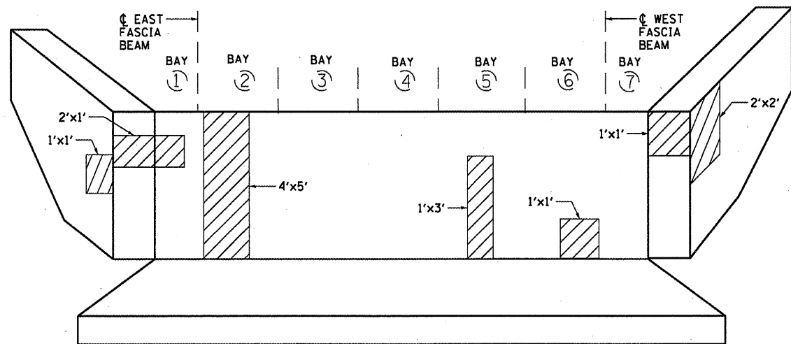
SOUTH ABUTMENT
