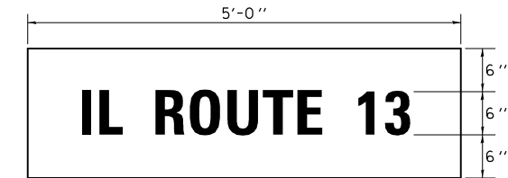
SIGN PANEL - TYPE 1 5'-0" x 1'-6" NE & SW MAST ARMS
