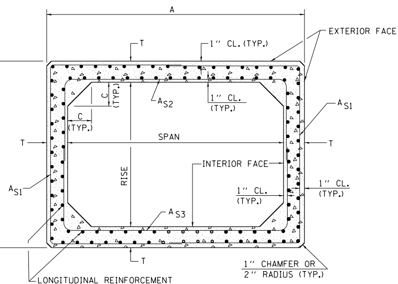
CROSS SECTION
