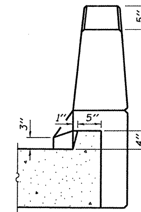
VIEW B-B
