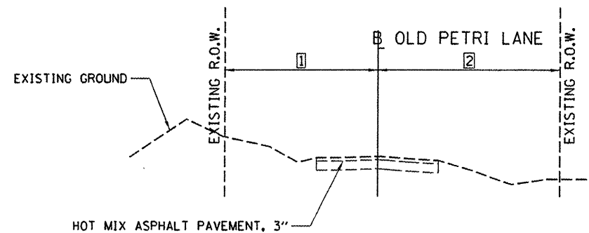
OLD PETRI LANE EXISTING TYPICAL SECTION STA. 500+76.00 TO STA. 501+45.00
