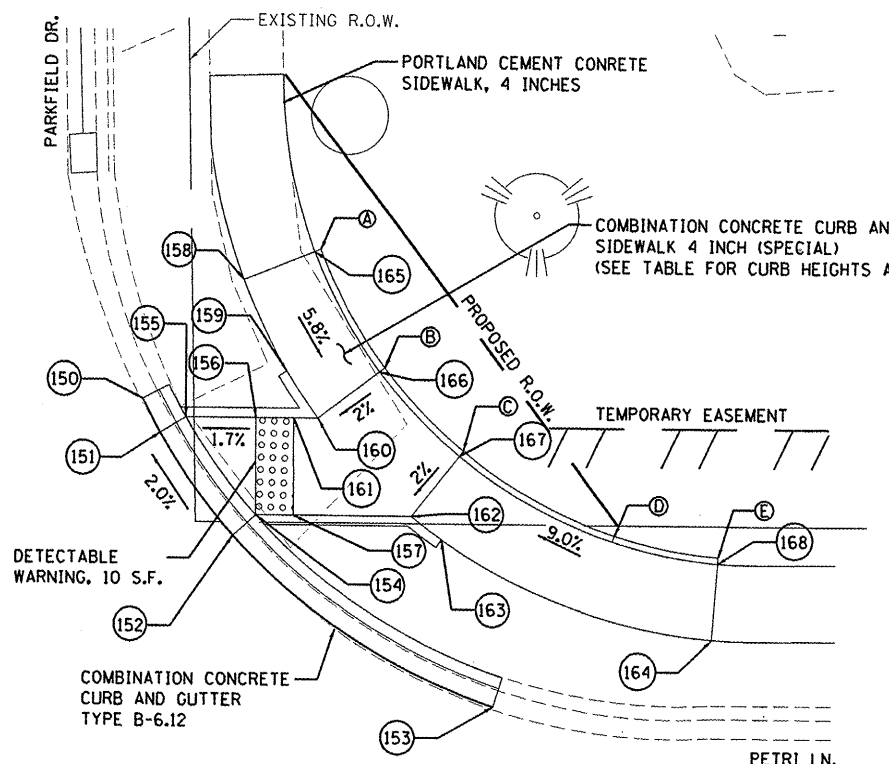
PETRI LN. AND PARKFIELD DR. NORTH EAST SIDEWALK RAMP SCALE: 1" = 5'
