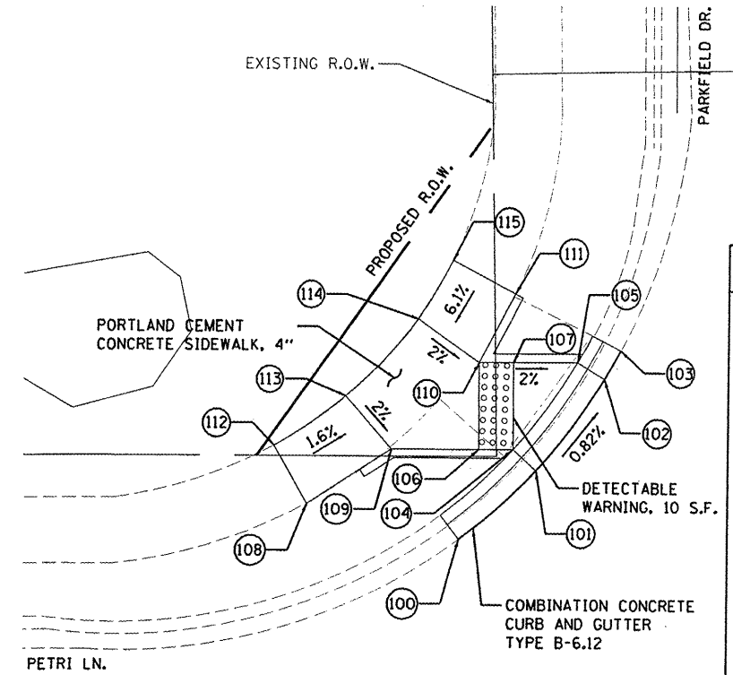
PETRI LN. AND PARKFIELD DR. NORTH WEST SIDEWALK RAMP SCALE: 1" = 5'
