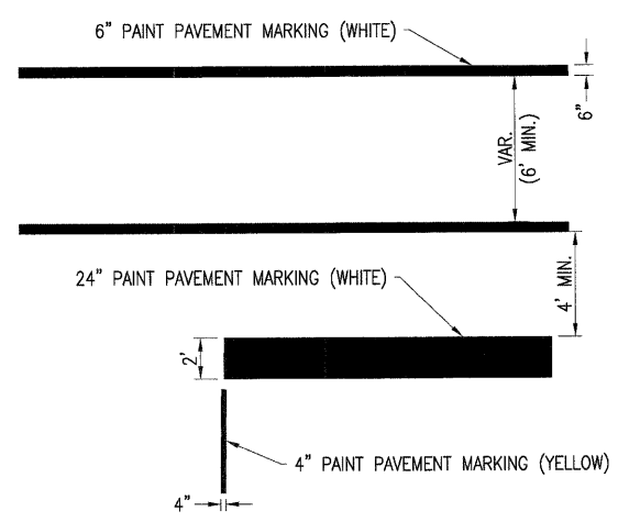
CROSSWALK, CENTERLINE & STOP BAR DETAIL SCALE: 1" = 5'
