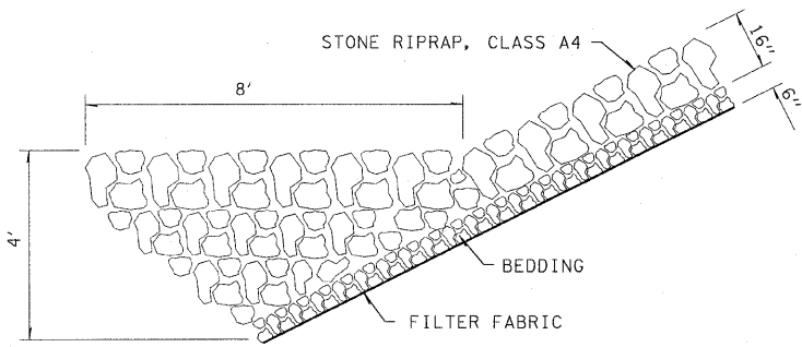
STONE RIPRAP ANCHOR DETAIL
