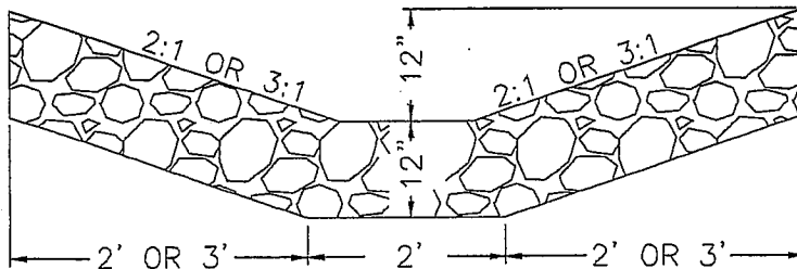
DETAIL OF AGGREGATE DITCH (SPECIAL)
