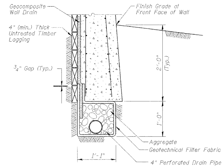
UNDERDRAIN DETAIL (Between Soldier Piles)
