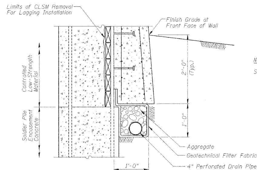
UNDERDRAIN DETAIL (At Soldier Piles)
