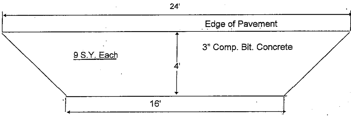
TYPICAL FIELD ENTRANCE
