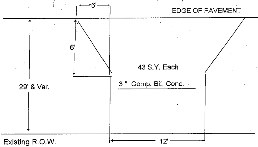
TYPICAL PRIVATE ENTRANCE
