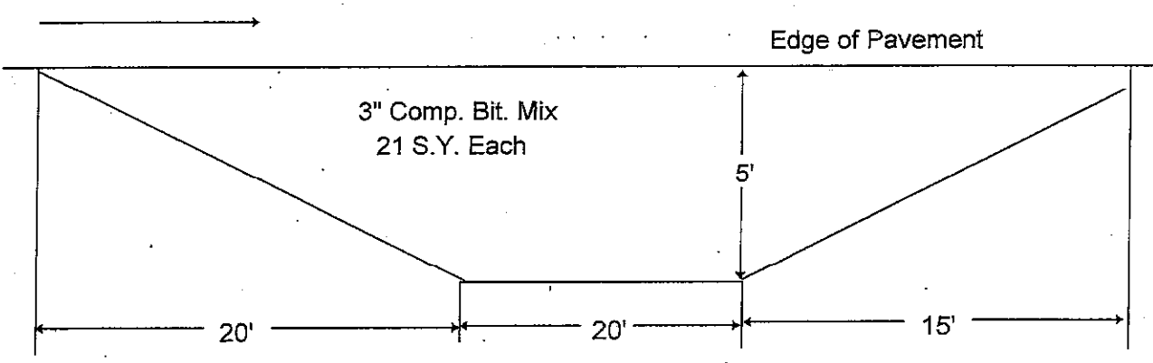
TYPICAL MAILBOX TURNOUT
