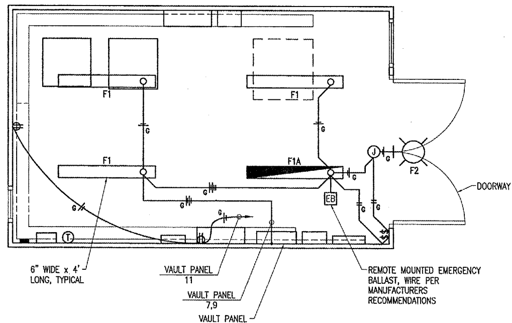
Vault Lighting & Receptacle Plan SCALE 1/2"=1'-0" 1 0 2 4 FEET
