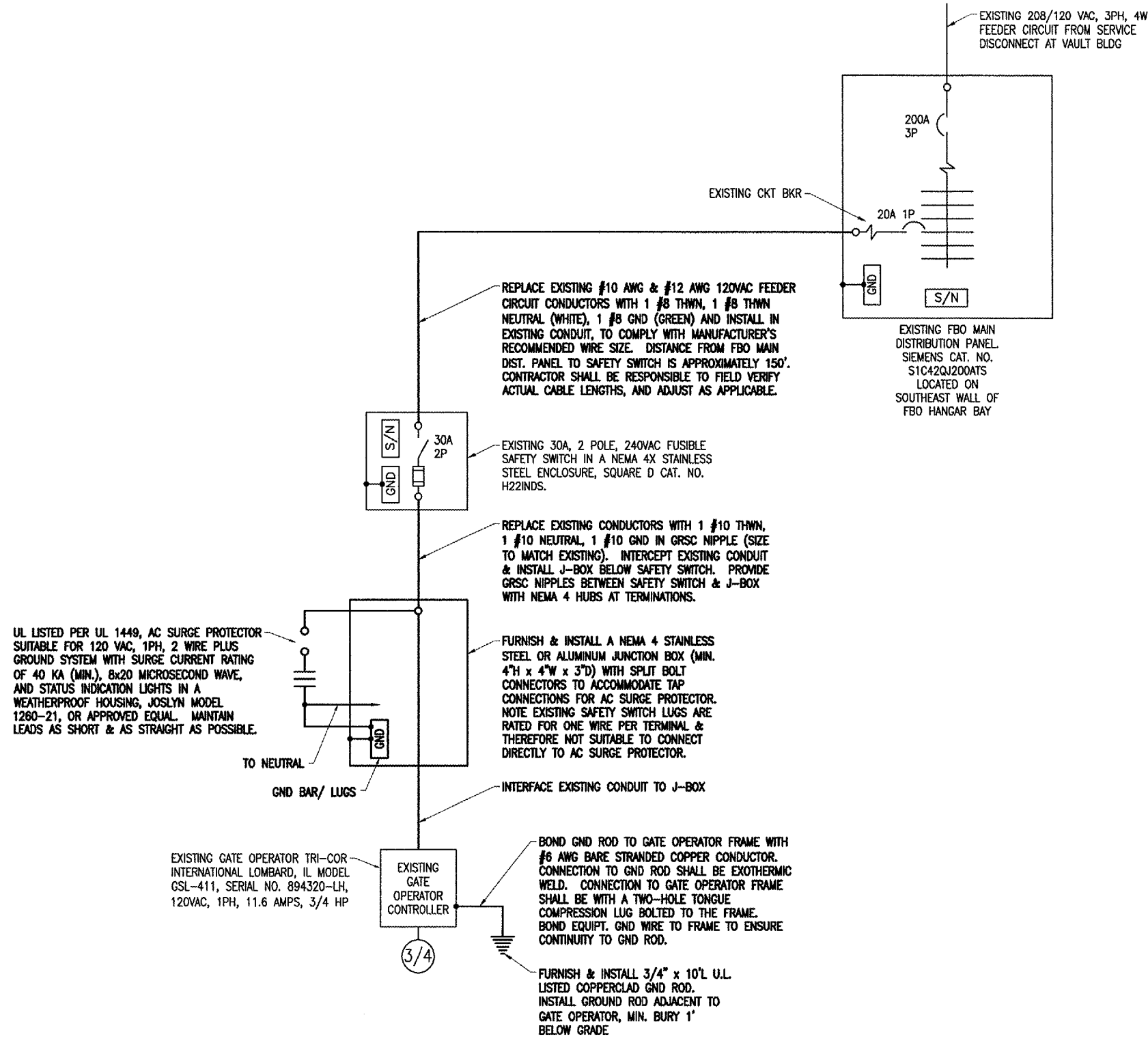
GATE NO. 3 ELECTRICAL ONE LINE
