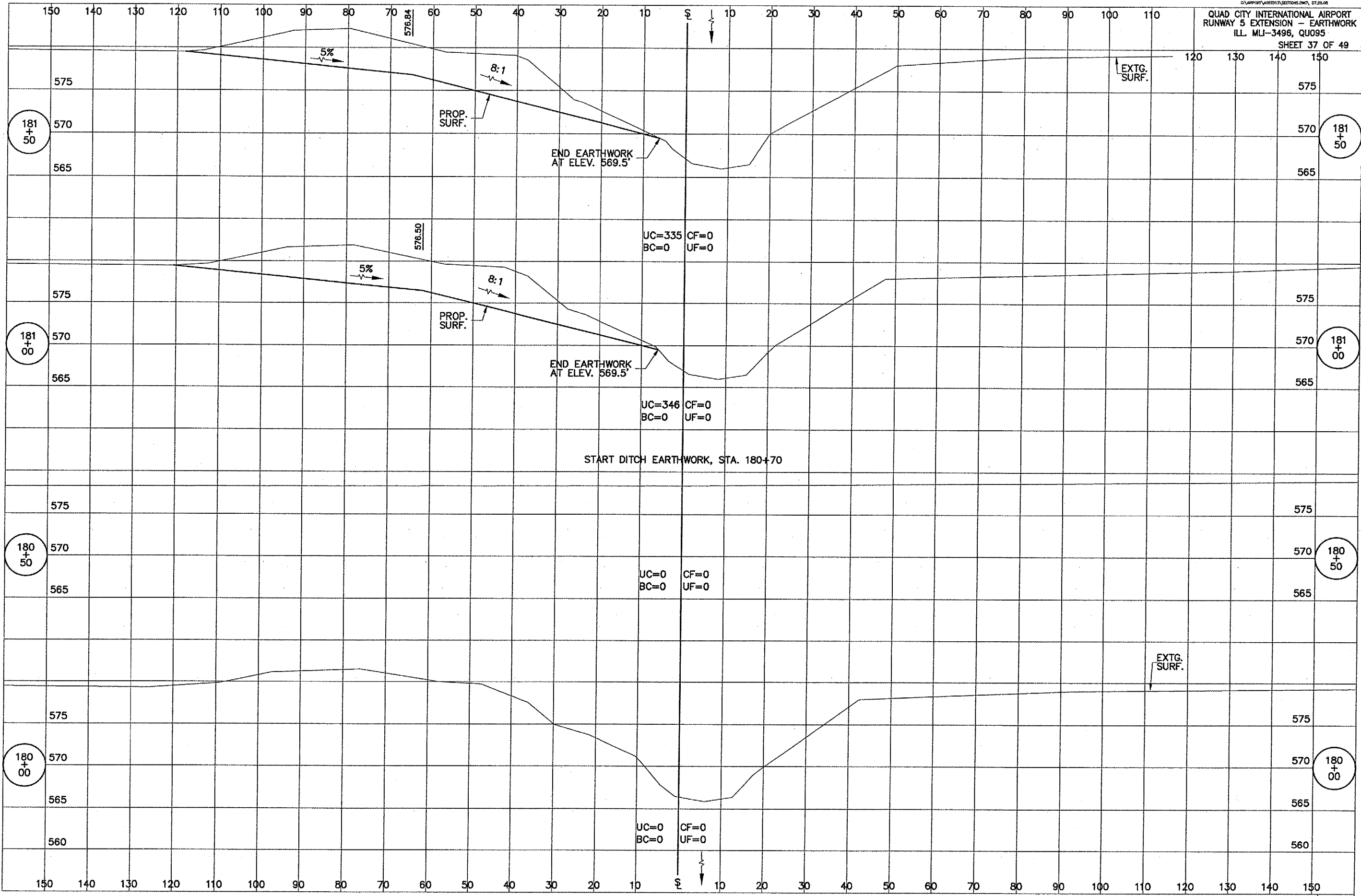
DITCH CROSS SECTIONS, STA 180+00 TO STA 181+50
