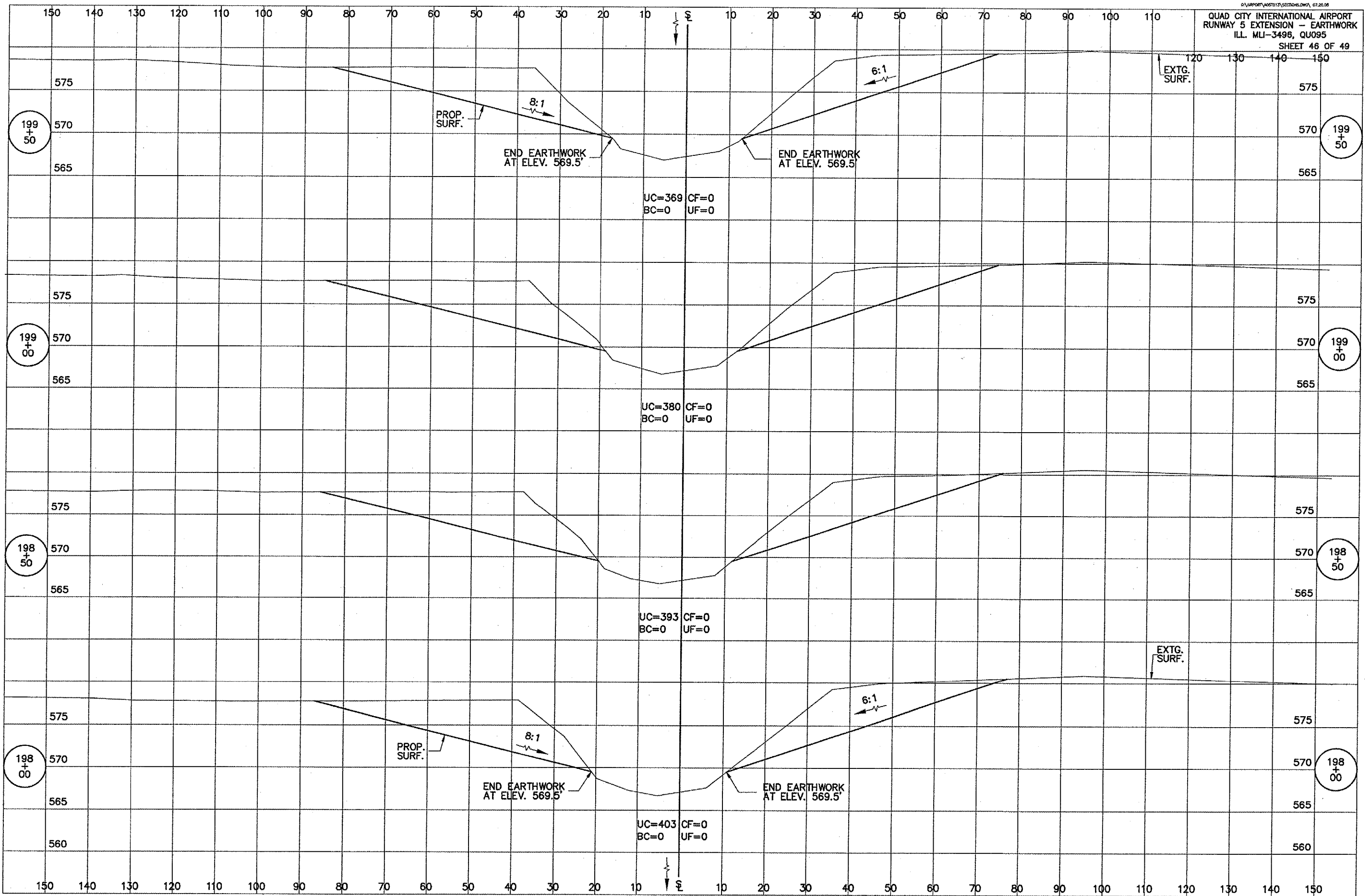
DITCH CROSS SECTIONS, STA 198+00 TO STA 199+50
