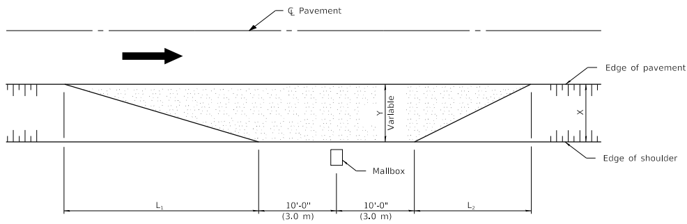
TYPICAL APPLICATION
