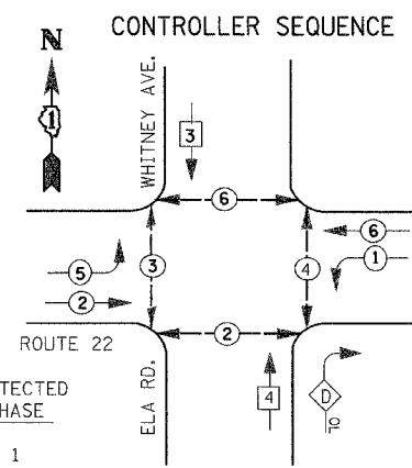
PHASE DESIGNATION DIAGRAM
