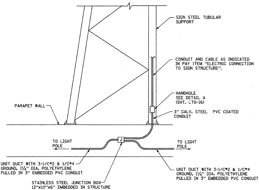
PROPOSED CANTILEVER TRUSS SIGN (WB) STA. 496+00 I-55 (LOOKING SOUTH) NOT TO SCALE
