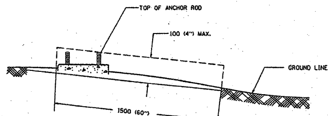
FOUNDATION EXTENSION DETAIL
