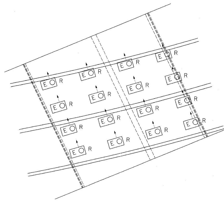
EXISTING UNDERPASS ENLARGED FIXTURE REMOVAL PLAN NOT TO SCALE
