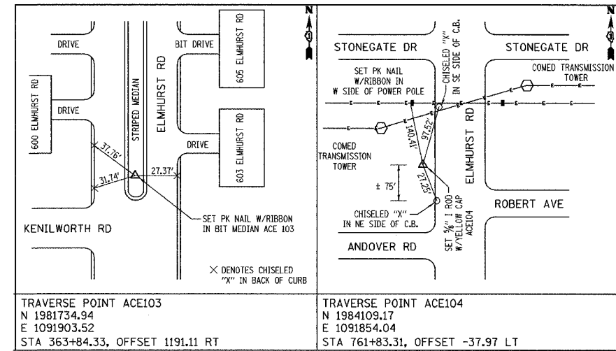
TRAVERSE POINT TIE DIAGRAMS (NOT TO SCALE)
