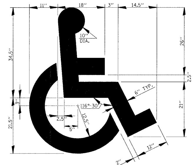
TYPICAL DETAIL FOR PAINTING HANDICAP MARKINGS
