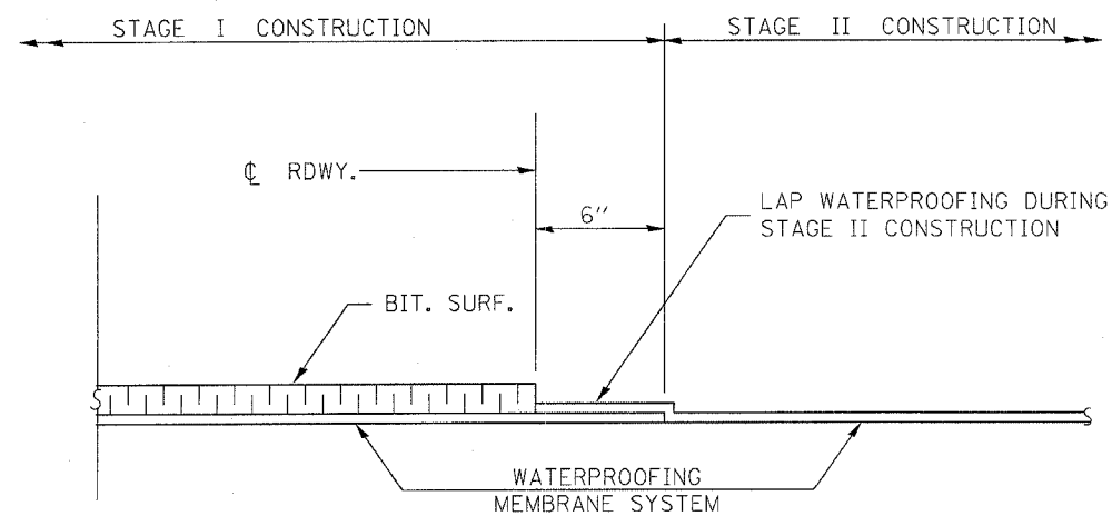
WATERPROOFING TREATMENT AT STAGE CONSTRUCTION
