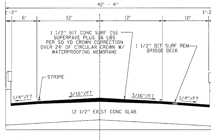
STRUCTURE NO. 038-0170 EAST BOUND
