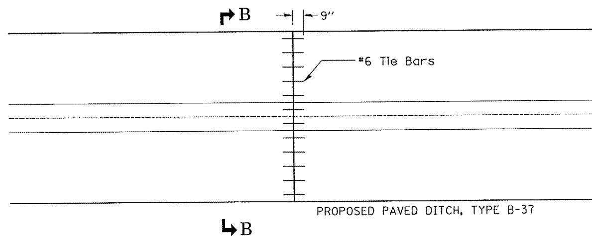
PLAN AT CONSTRUCTION JOINTS
