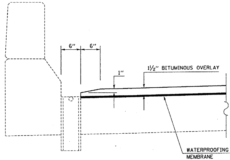
DETAIL OF DRAIN AT CURB
