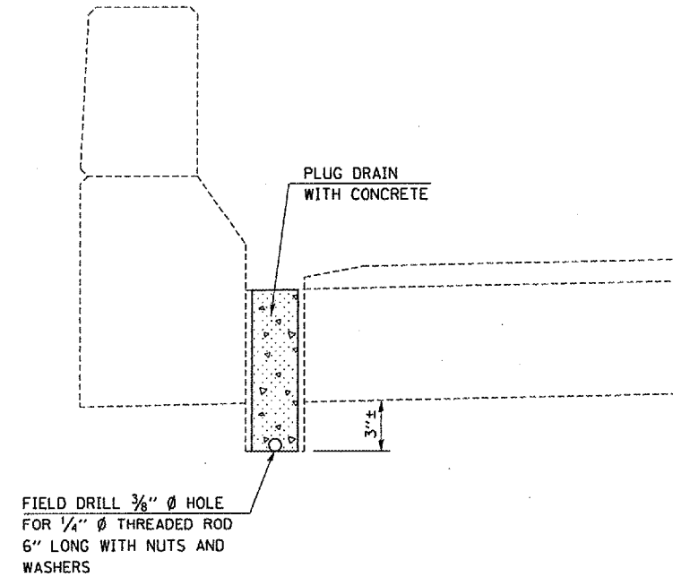
DRAIN ELIMINATION DETAIL SECTION AT DRAIN
