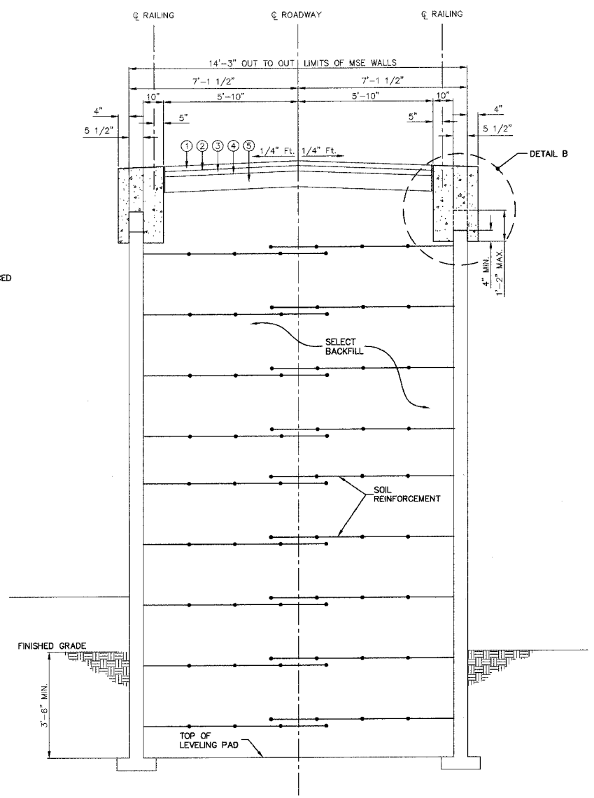
SECTION THROUGH MSE WALLS
