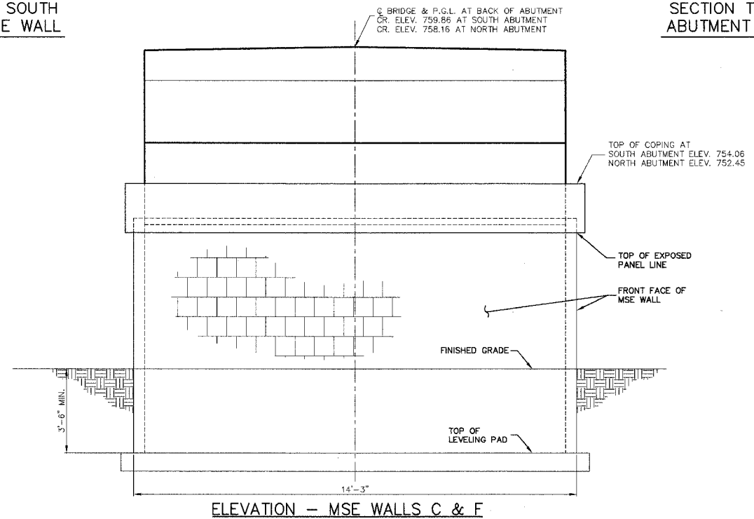
ELEVATION - MSE WALLS C & F
