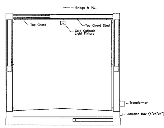
BRIDGE CROSS SECTION
