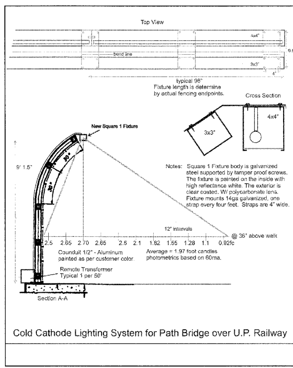
BRIDGE CROSS SECTION
