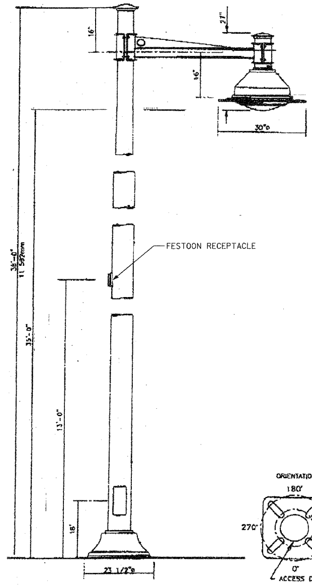
LIGHT POLE, ORNAMENTAL NOT TO SCALE
