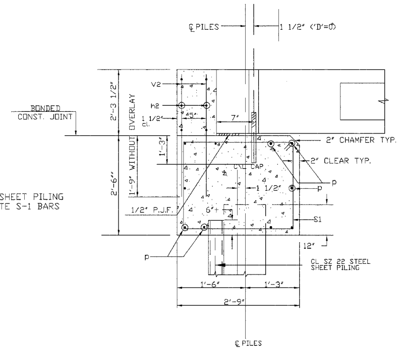
SECTION THROUGH BOTH ABUTMENTS
