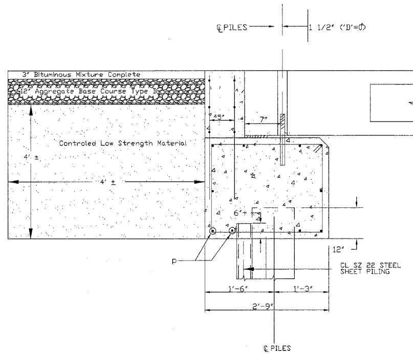
FILL AT BOTH ABUTMENTS
