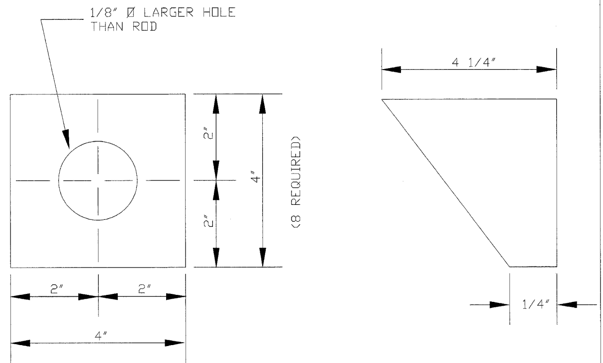
BEVELED WASHER DETAIL (8 REQUIRED)
