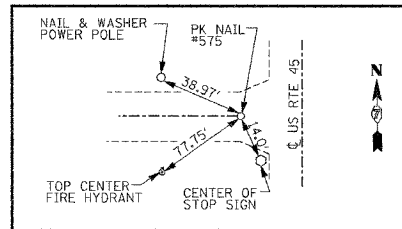
TR1725N STA 10+00.00 PK NAIL #575
