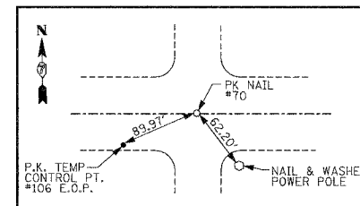
TR1550N STA 10+00.00 PK NAIL #70
