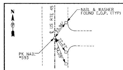
TR1500N STA 10+00.00 PK NAIL #593
