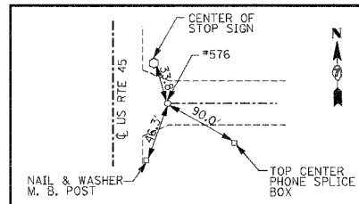
TR1700N STA 10+00.00 #576 60 SPIKE
