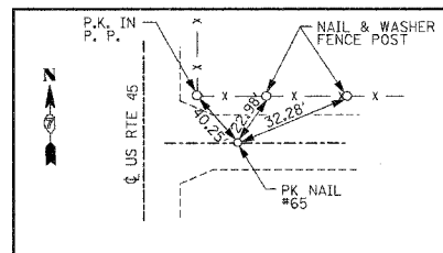
TR1625N STA 10+00.00 PK NAIL #65
