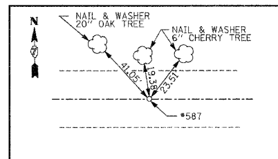
TR1600N STA 5+00.00 #587 SET 60 SPIKE
