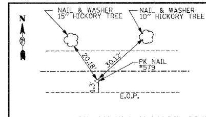
TR1650N PI STA 8+26.92 PK NAIL #579
