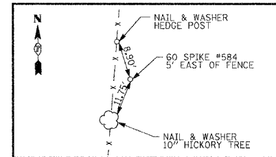
TR1650N STA 10+00.00 #584 60 SPIKE
