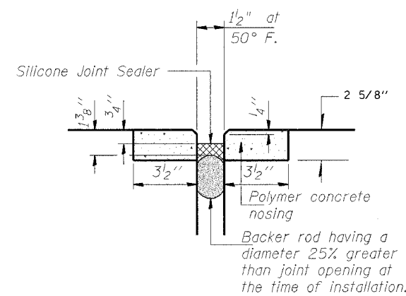
SILICONE JOINT SEALER DETAIL DETAIL B
