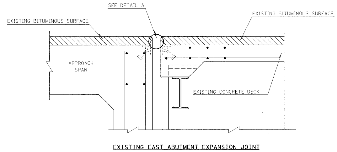
EXISTING EAST ABUTMENT EXPANSION JOINT
