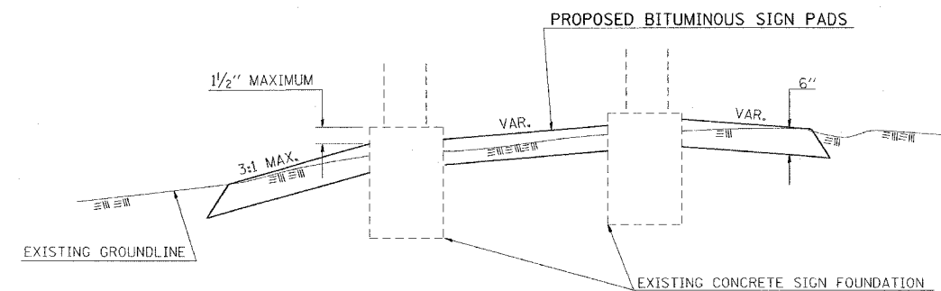
SECTION B-B
