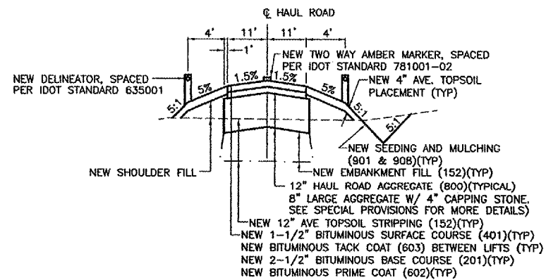
TYPICAL SECTION D-D HAUL/PERIMETER ROAD NOT TO SCALE
