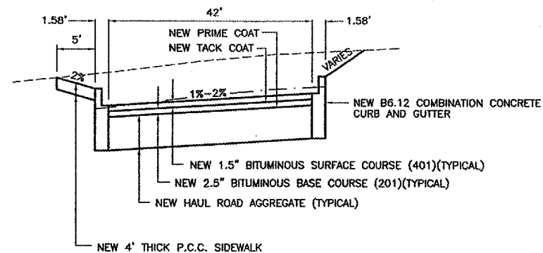
TYPICAL SECTION E-E AUTO PARKING LOT NOT TO SCALE
