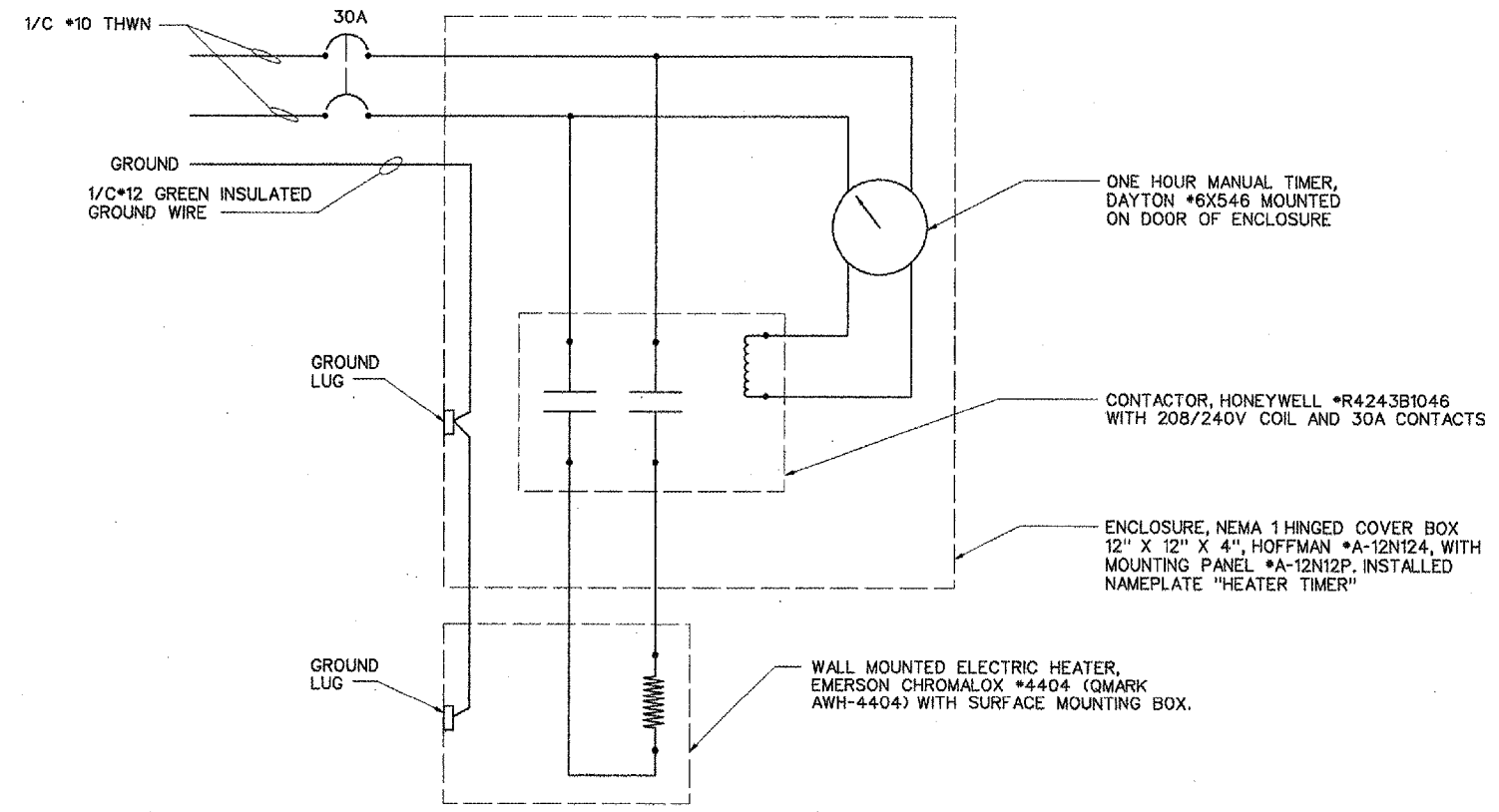
HEATER AND TIMER WIRING
