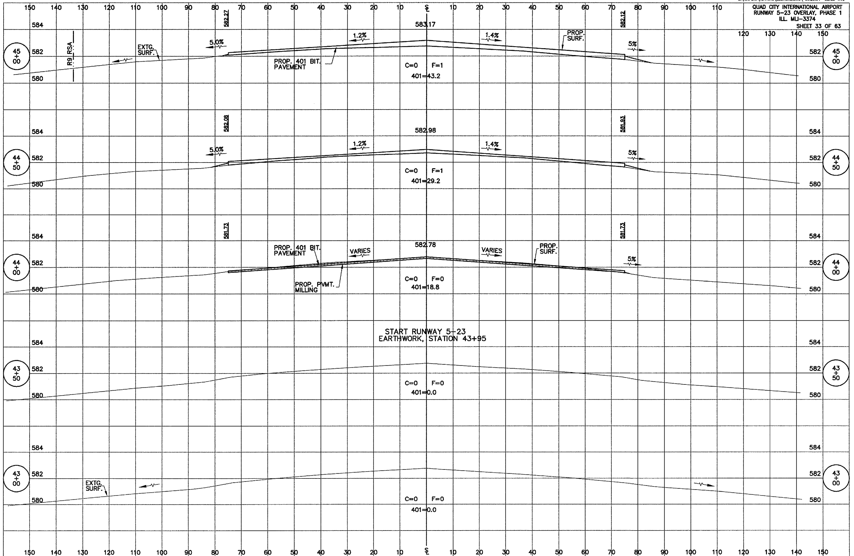
RUNWAY 5-23 OVERLAY CROSS SECTIONS, STA 43+00 TO STA 45+00
