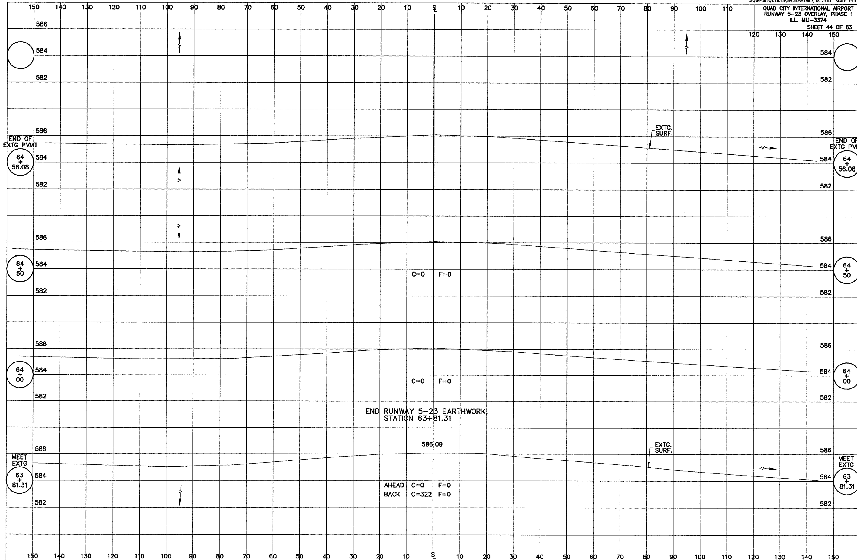
RUNWAY 5-23 OVERLAY CROSS SECTIONS, STA 63+81.31 TO STA XX+XX
