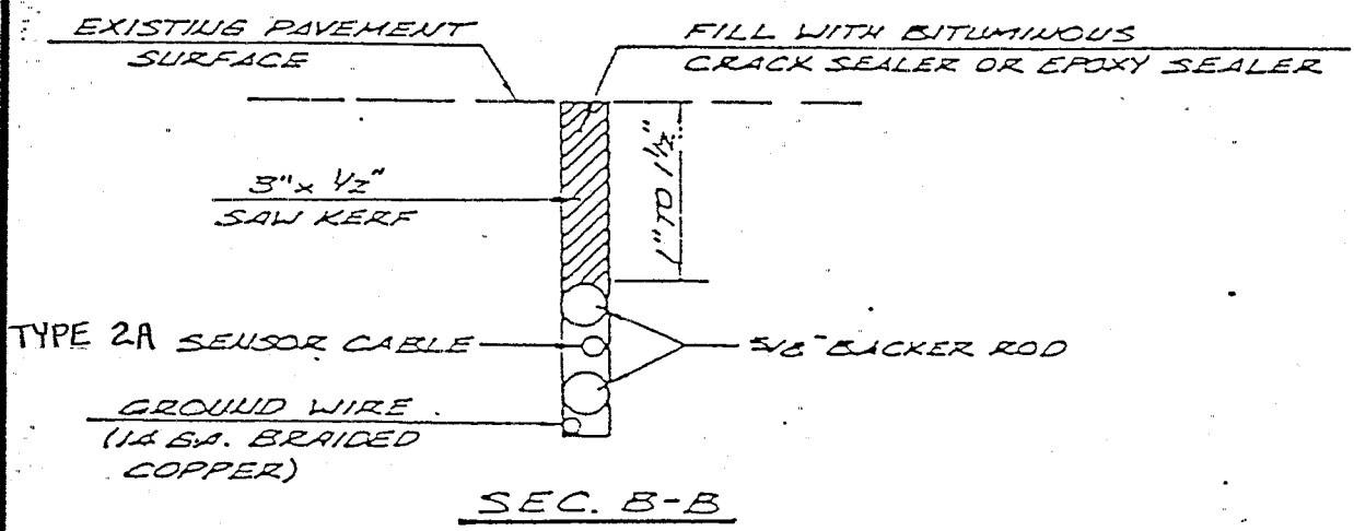
TYPICAL SENSOR HEAD AND CABLE INSTALLATION
