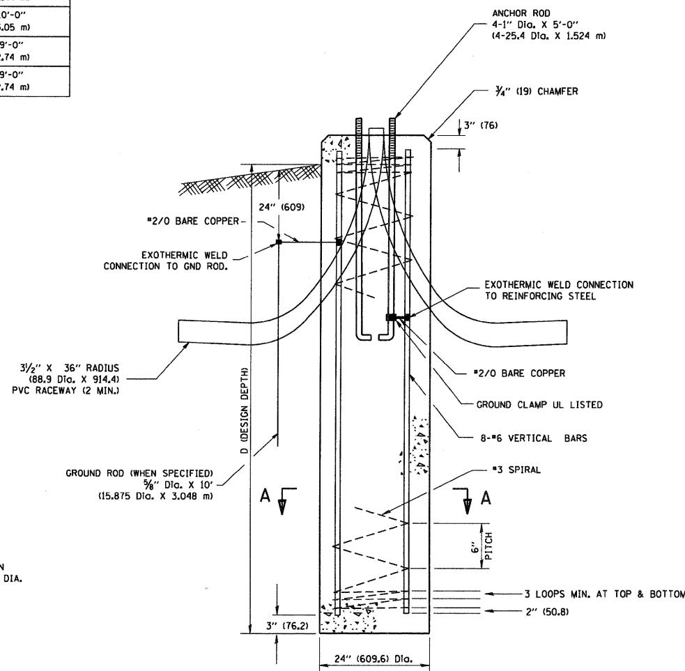
FOUNDATION DETAIL
