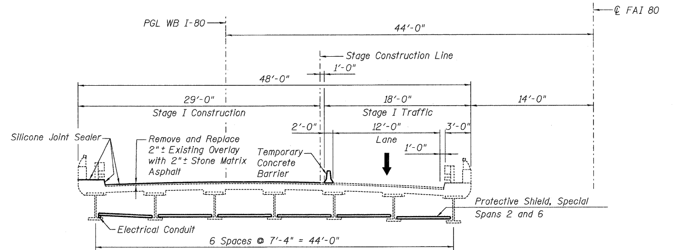
STAGE I CONSTRUCTION & TRAFFIC (Looking East)
